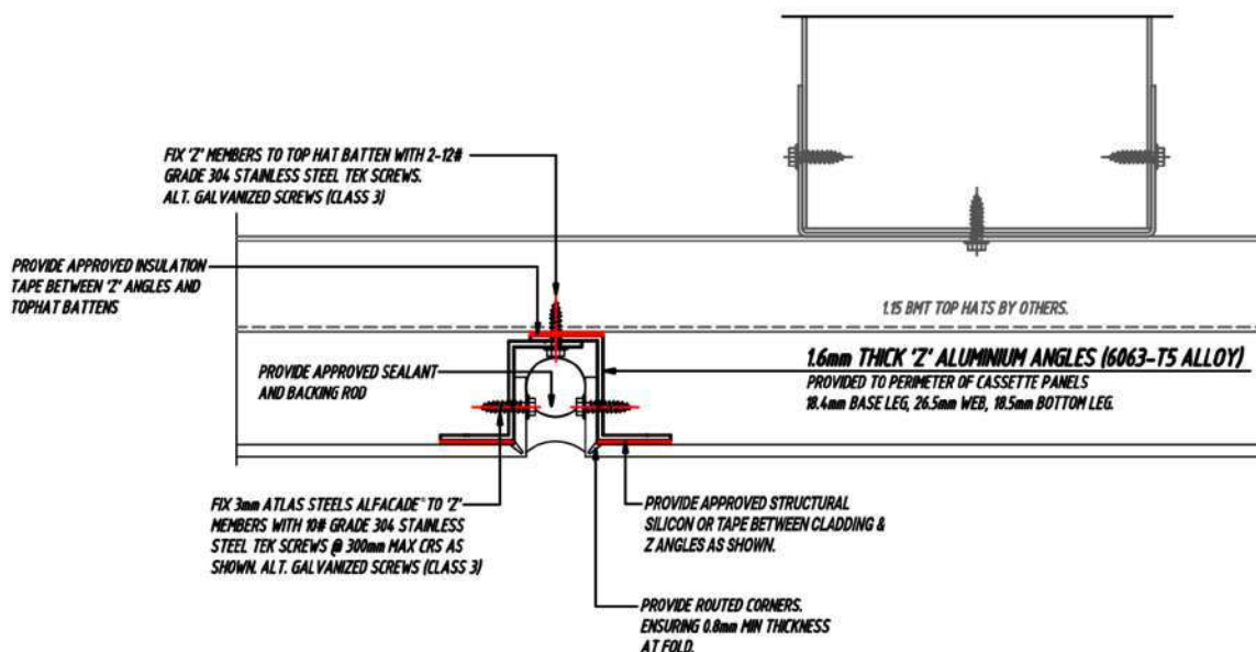
DETAIL 1/S1 SCALE 1/125
