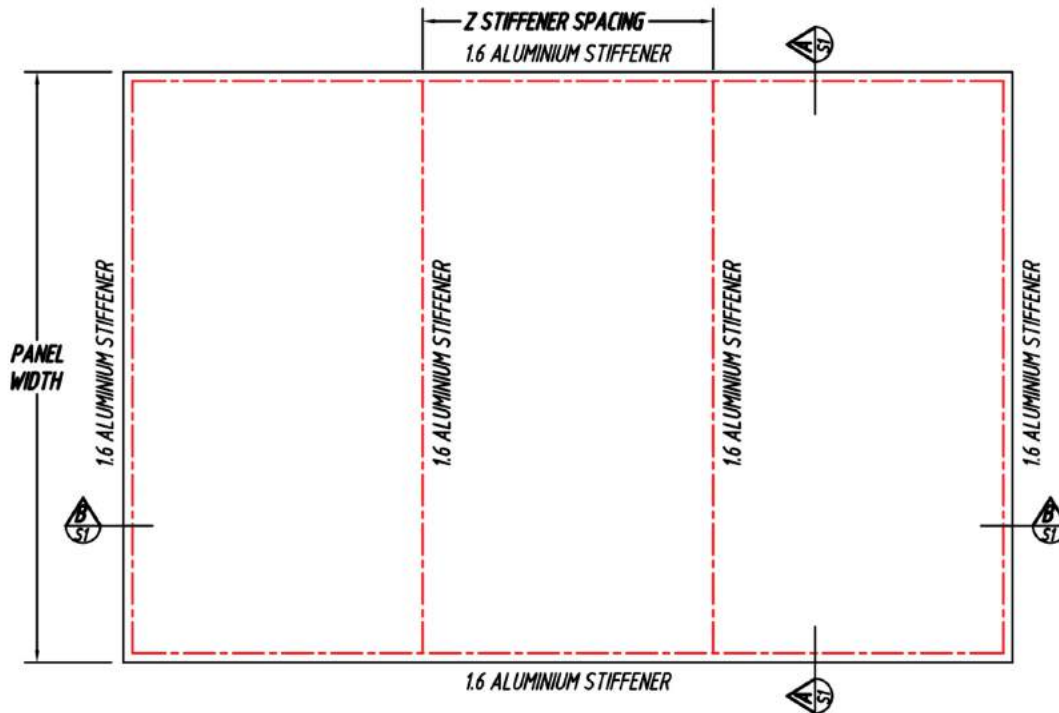
TYPICAL PANEL LAYOUT SCALE 1:10
