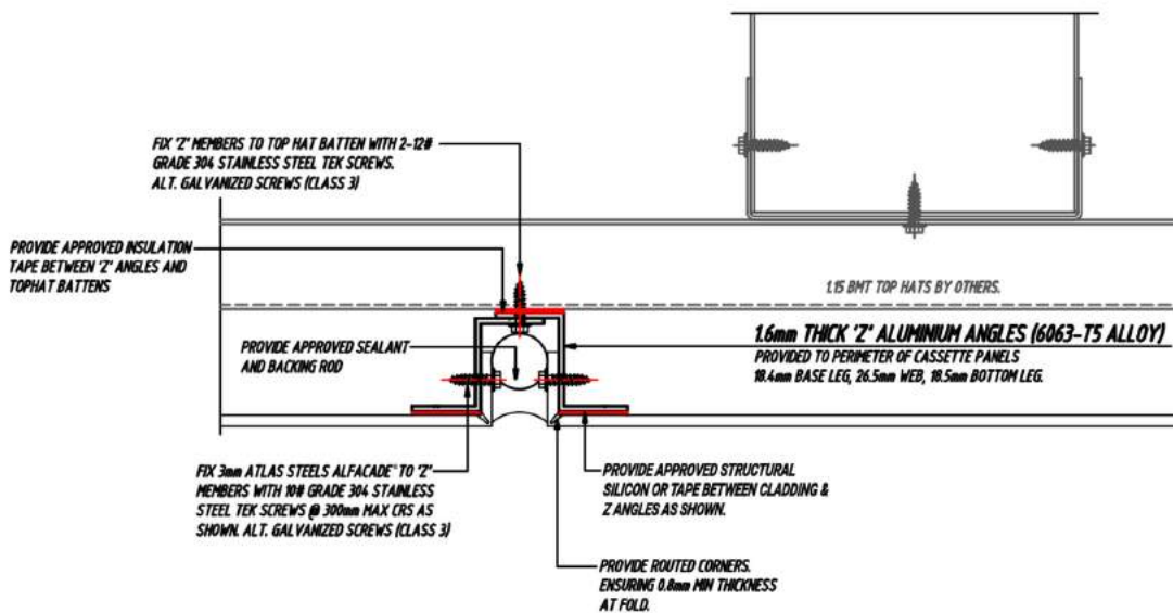
DETAIL 1/S1 SCALE 1:25
